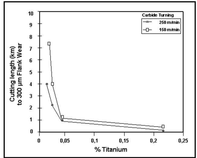
Figure 15: The addition of titanium dramatically reduces the tool life of compacted graphite iron during carbide turning
