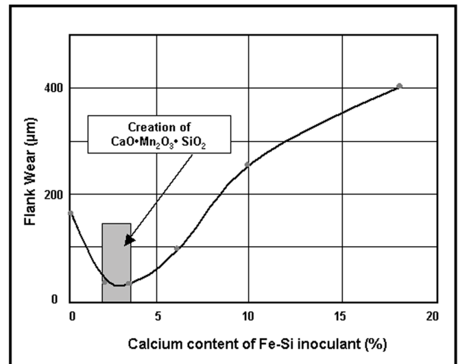
Figure 16: A gray iron inoculant containing 2-3% calcium optimizes the ability to form a protective layer on a TiC coated insert [7]
