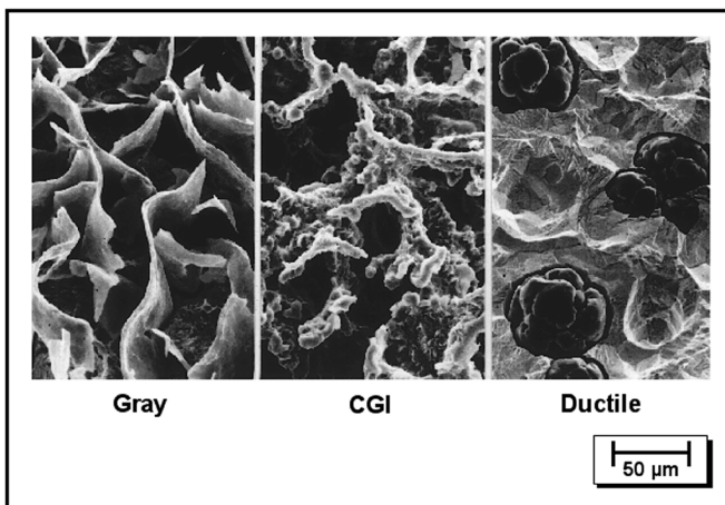
Figure 2: Deep-etched scanning electron micrographs show the three-dimensional shape of the graphite
