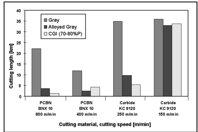
Figure 5: Tool life for convention gray iron, alloyed gray iron, and 70-80% pearlitic CGI for PCBN and carbide turning
