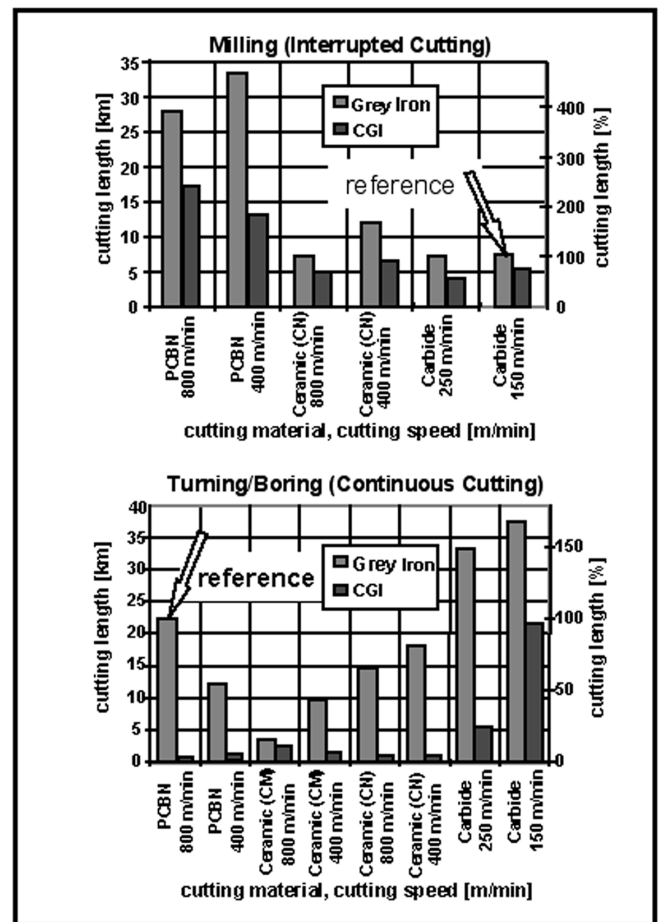
Figure 3: Comparative tool life for different tool materials in interrupted (milling) and continuous (turning/boring) cutting of 70-80% pearlitic CGI and gray iron
