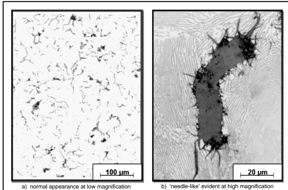
Figure 11: The use of antimony for pearlite stabilization causes spikes on the graphite particles
