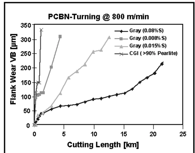
Figure 13: The machinability of gray cast iron gradually decreases as the sulfur content is reduced from, normal gray iron levels (0.08%S) to normal CGI levels (0.008%S)
