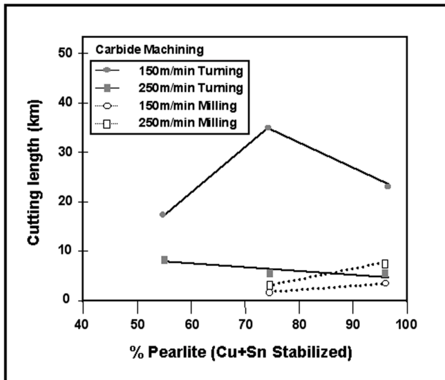
Figure 8: The effect of pearlitic content on tool life during carbide milling and turning. The pearlite was stabilized by additions of copper and tin
