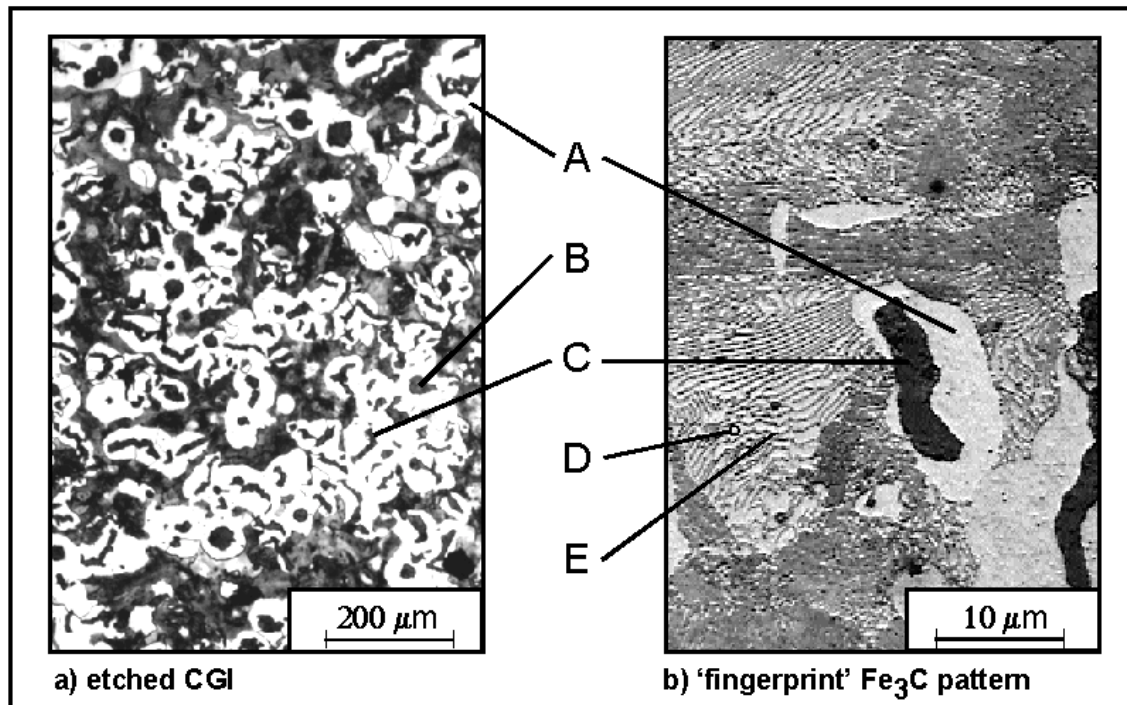
Figure 7: The pearlite phase is an ordered layering of ferrite and \text{Fe}_3\text{C} plates (A: free ferrite, B: pearlite, C: graphite, D: ferrite band, E: \text{Fe}_3\text{C} plate)
