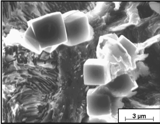
Figure 14: Cubic titanium carbonitride inclusions are harder than tungsten carbide and significantly increase abrasive tool wear
