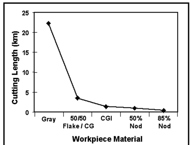
Figure 4: The influence of graphite shape on tool life for PCBN turning at 800 m/min
