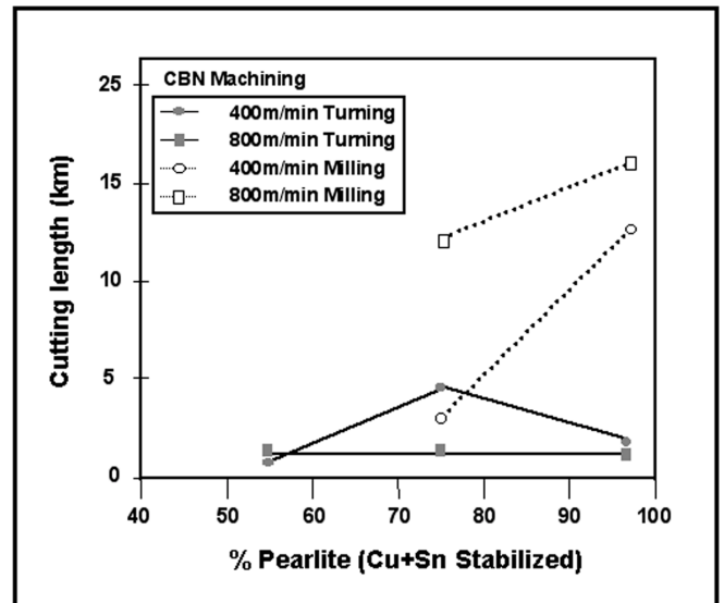
Figure 9: The effect of pearlitic content on tool life during CBN milling and turning. The pearlite was stabilized by additions of copper and tin
