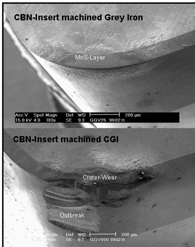
Figure 12: Protective MnS layers form on the cutting edge of PCBN inserts when cutting gray iron at high speeds. In contrast, inserts used for CGI exhibit abrasive wear
