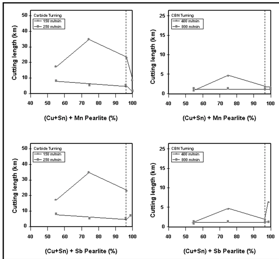
Figure 10: The effect of an incremental increase from 97.5% pearlite (Cu+Sn) to 99% (Sb-CGI) and 100% (Mn-CGI) pearlite on tool life during carbide and CBN turning
