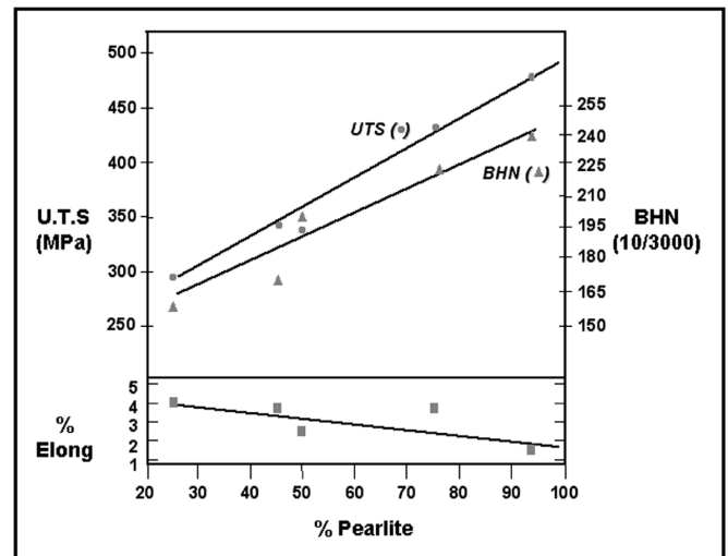
Figure 6: The effect of pearlite content on the ultimate tensile strength, hardness and elongation of 0-10% nodularity CGI in as-cast 25mm diameter test bars After [1]
