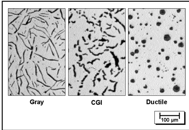
Figure 1: Gray iron, compacted graphite iron and ductile iron are differentiated by the shape of the graphite particles
