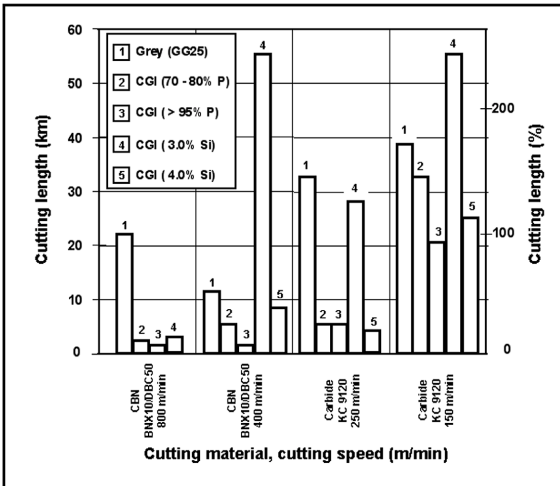
Figure 17: The effect of silicon content on CGI tool life during CBN and carbide turning
